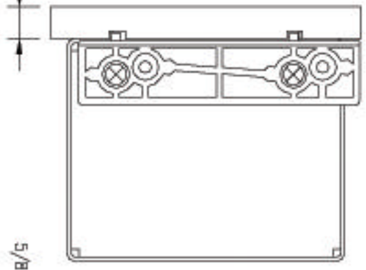
SIDE VIEW 1/2" DRYWALL FITTING
