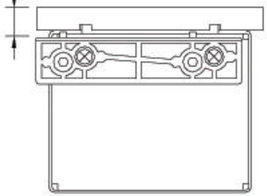
SIDE VIEW 5/8" DRYWALL FITTING
