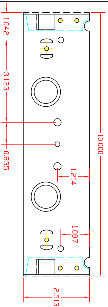
BACK VIEW
