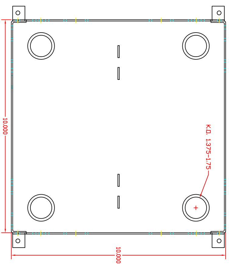
TOP VIEW
